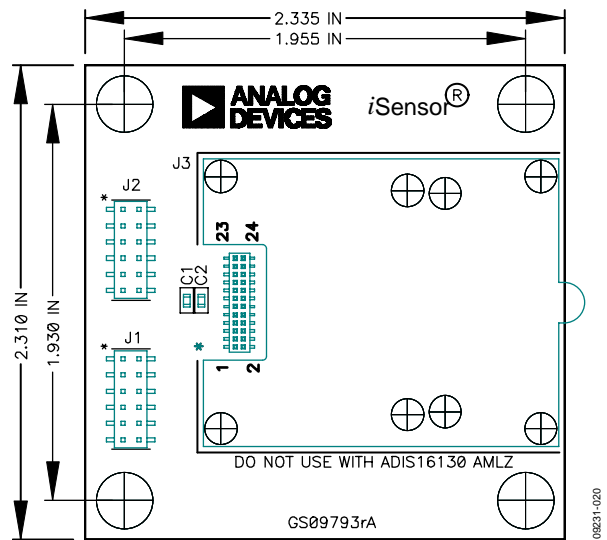
Figure 23. Physical Diagram for the ADIS16133/PCBZ
