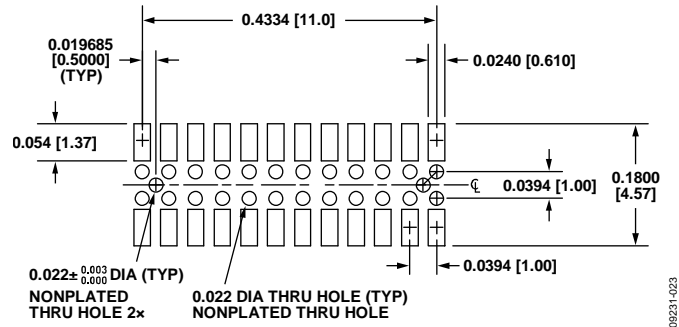
Figure 26. Suggested Layout and Mechanical Design for the Mating Connector
