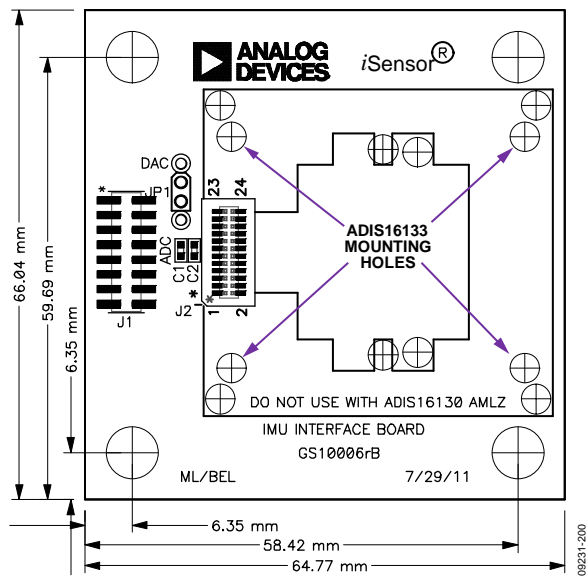
Figure 21. Physical Diagram for the Current ADIS16133/PCBZ
